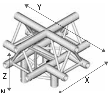
90° CROSS 5 WAYS TOP APEX
