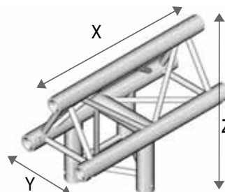
90° CORNER 3 WAYS "T" VERTICAL TOP APEX
