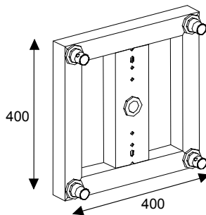
TB 95443 Professional HD 40 Sliding Corner Block
