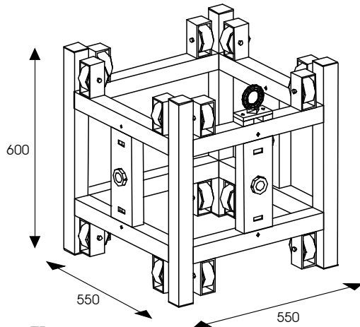
TB 95443 Professional HD 40 Sliding Corner Block
