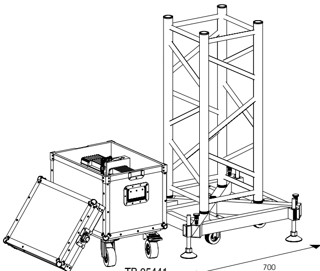
TB 95441 Professional HD 40 steel base
