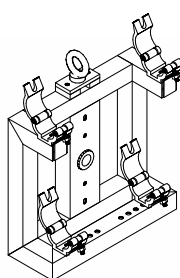
TB 9840 Side Flange for Roof Systems with 40x40 section Truss Weight kg 8,5
