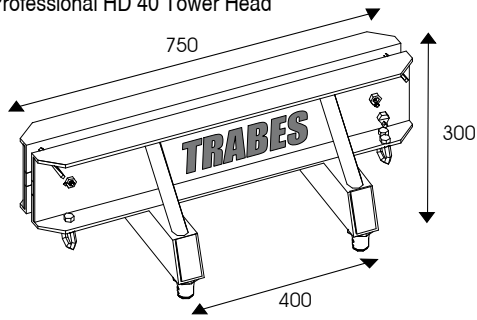
TB 95444 Professional HD 40 Tower Head
